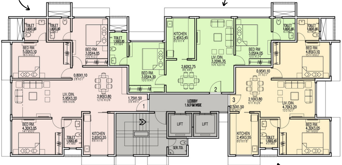
6TH FLOOR PLAN.
