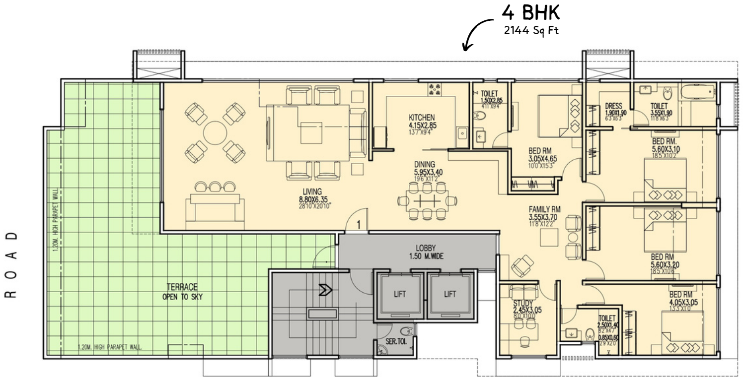
7TH FLOOR PLAN.
