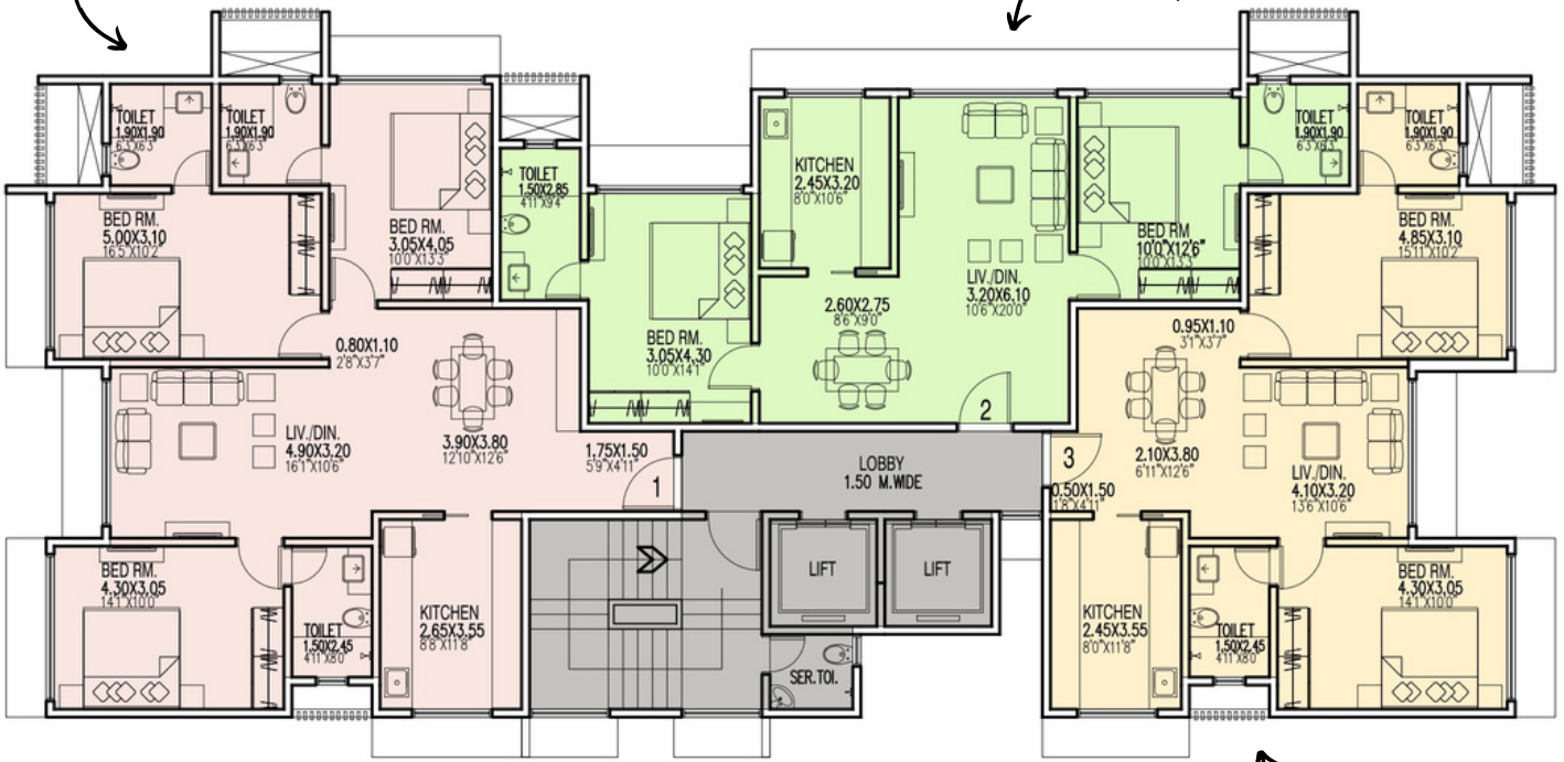
2ND TO 4TH FLOOR PLAN.
